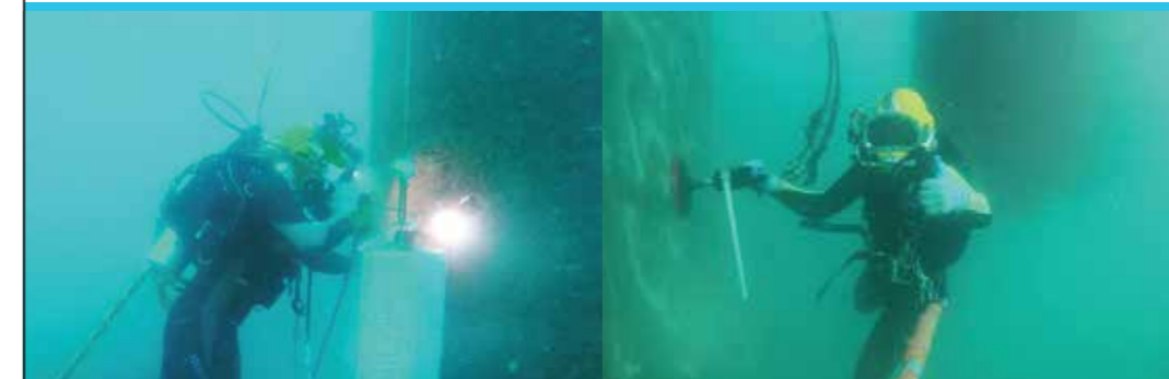
Cathodic Protection Installation
